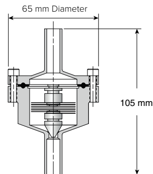
Model TC-R Repairable With Bolted Body and Cap 1/2" and 3/4" Tube End Connections
