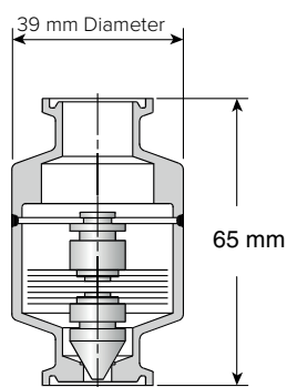
Model TC-S Sealed 1/2" and 3/4" Sanitary End Connections
