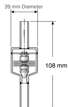
Model TC-S Sealed 1/2" and 3/4" Tube End Connections
